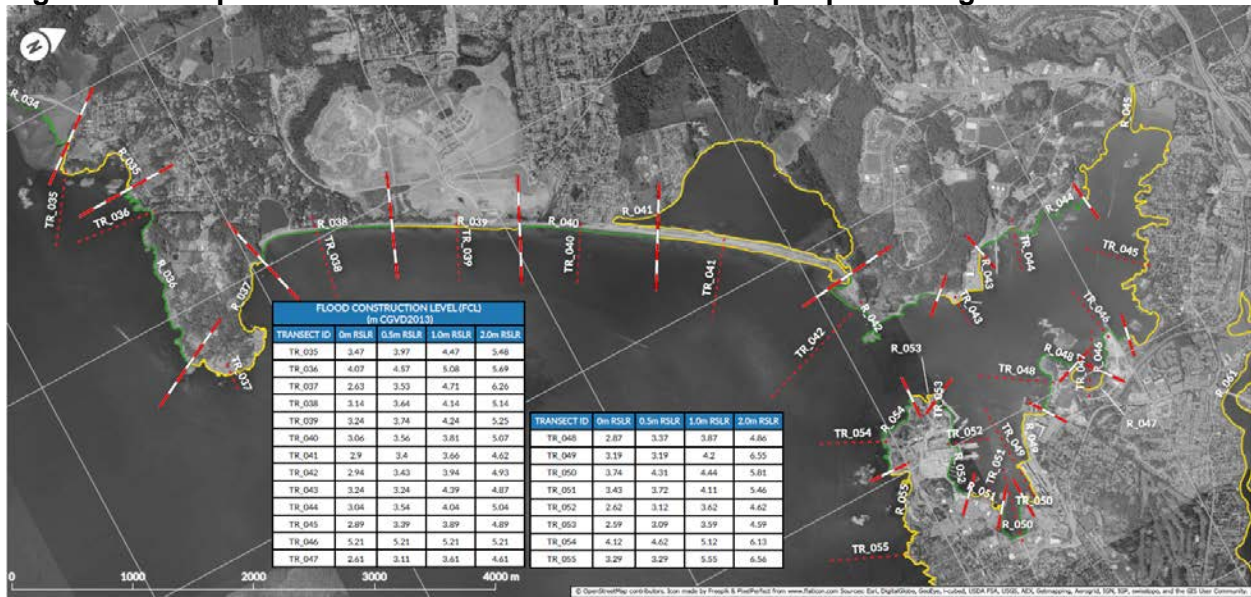
Figure 2: Example of SLR Flood Construction Level Map representing 21 Transects
