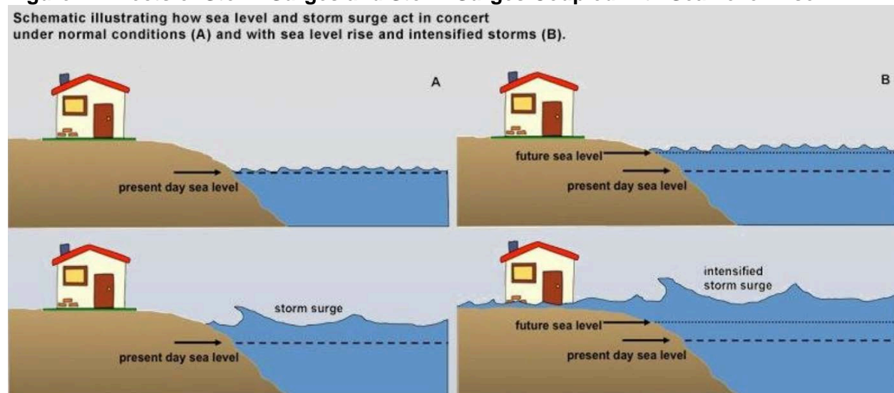
Figure 1: Effects of Storm Surges and Storm Surges Coupled with Sea Level Rise
