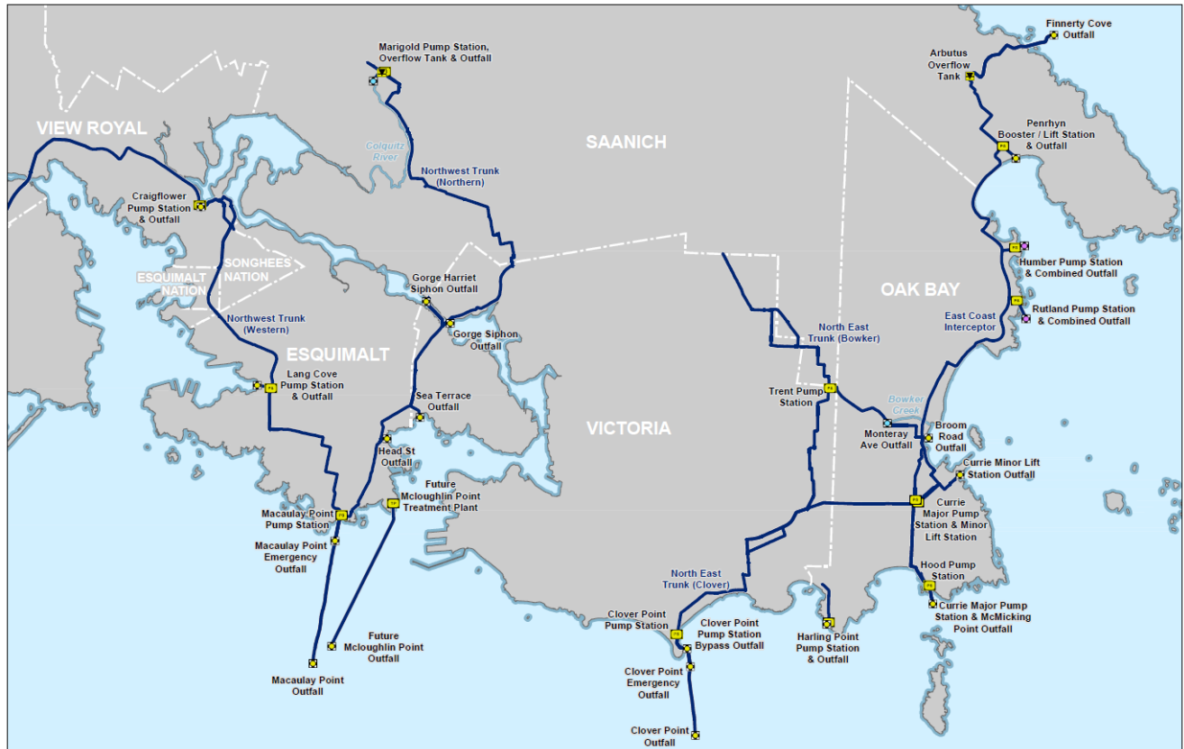
Figure 2: CRD's Two Major Regional Trunk Sewer Systems and Outfalls in the Core Area
