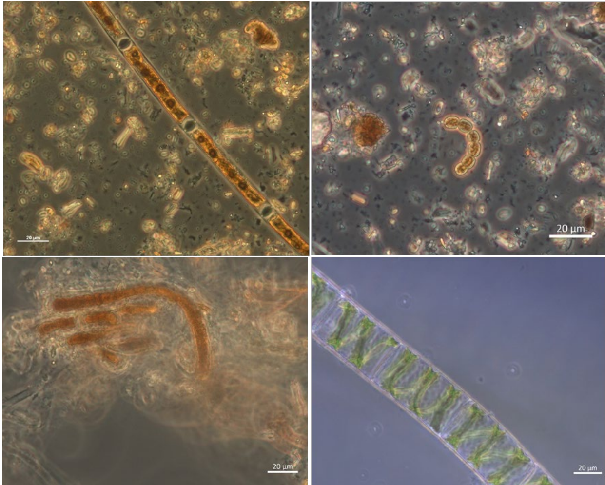
Figure 18 Some Periphyton Recorded in Leech Watershed
