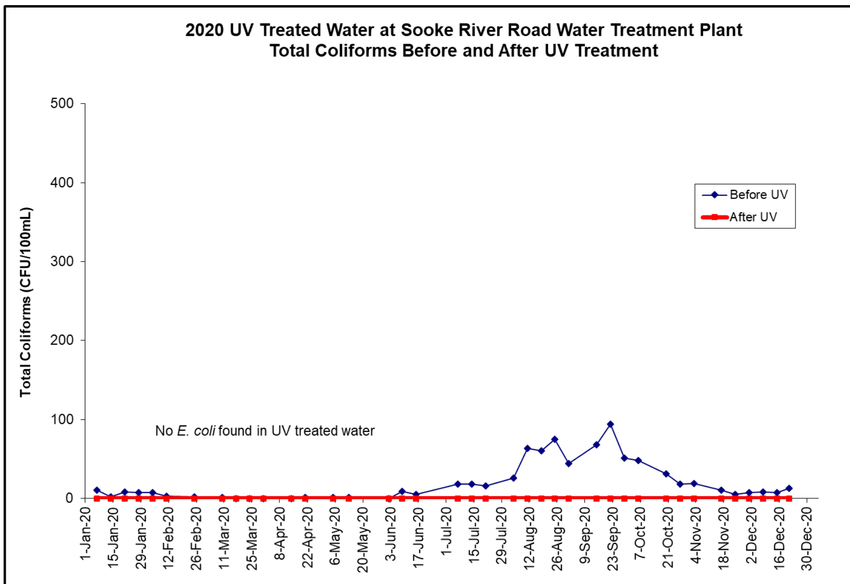
Figure 33 2020 UV Treated Water at Sooke River Road Water Treatment Plant Total Coliforms Before and After UV Treatment
