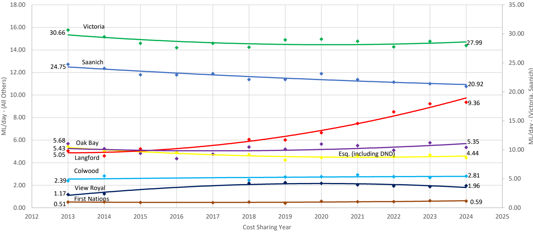
Average Dry Weather Flow (ADWF) Trends for Core Area Sewer Participants
